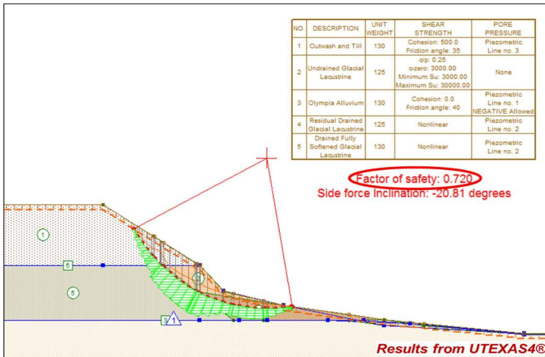
Figure 3.7: Stability Analysis for 2014 Landslide – Post-Failure of Lower Slope (from Gilbert et al. 2016)
