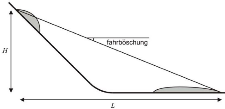
Figure 2.1: Definition of fahrböschung or angle of reach (from McDougall, 2006)
