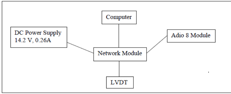
Figure 4.17: Data Acquisition System for Axial Displacement
