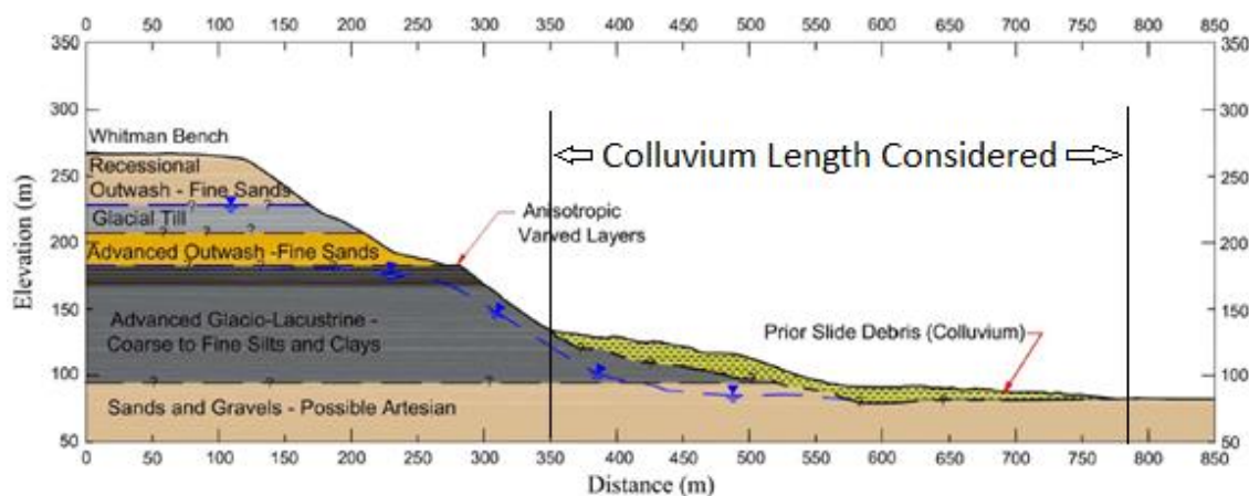
Figure 4.1: Slope Cross Section at Location in Figure 3.3 prior to 2014 Landslide (from Stark et al., 2017)
