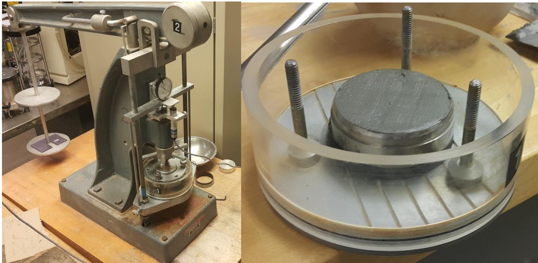
Figure 4.16: (a) Loading Frame, and (b) Consolidometer Used
