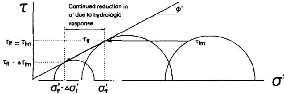
Figure 2.12: Stress Transfer Schematic due to Hydrologic Response
