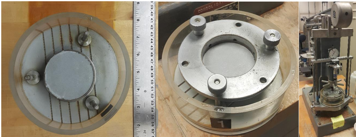
Figure 4.23: Specimens in Consolidometer and Consolidation Loading Frame
