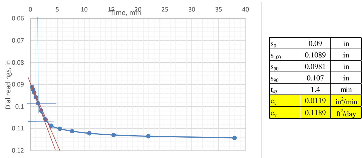
Figure 4.29: Square Root of Time Method for S1 Specimen Under 500 psf Vertical Stress
